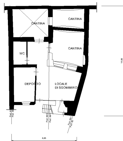
Piano terra
